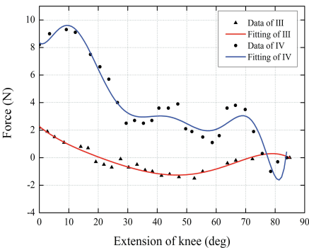
(b) The brace force in extension
