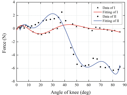
(a) The brace force in flexion
