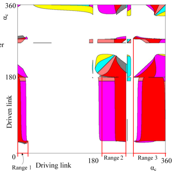
(b) The feasible solution region
