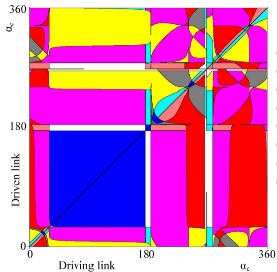
(a) Spherical 4R linkage solution region
