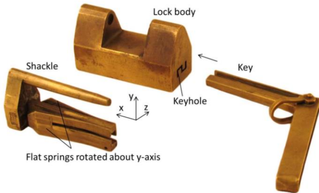
(a) Open keyhole padlock
