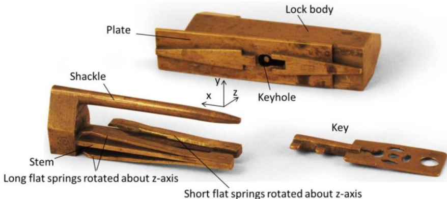
(b) Hidden keyhole padlock
