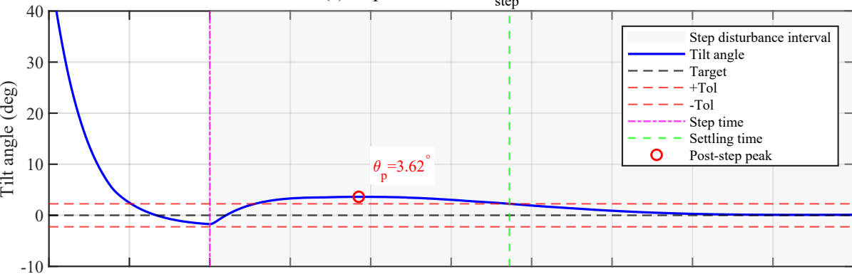
(b) Step disturbance: F_{\text{step}} = 20 \text{ N}
