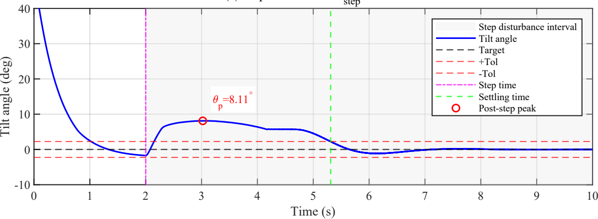
(c) Step disturbance: F_{\text{step}} = 30 \text{ N}
