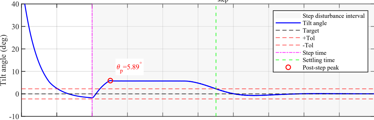
(c) Step disturbance: F_{\text{step}} = 30 \text{ N}
