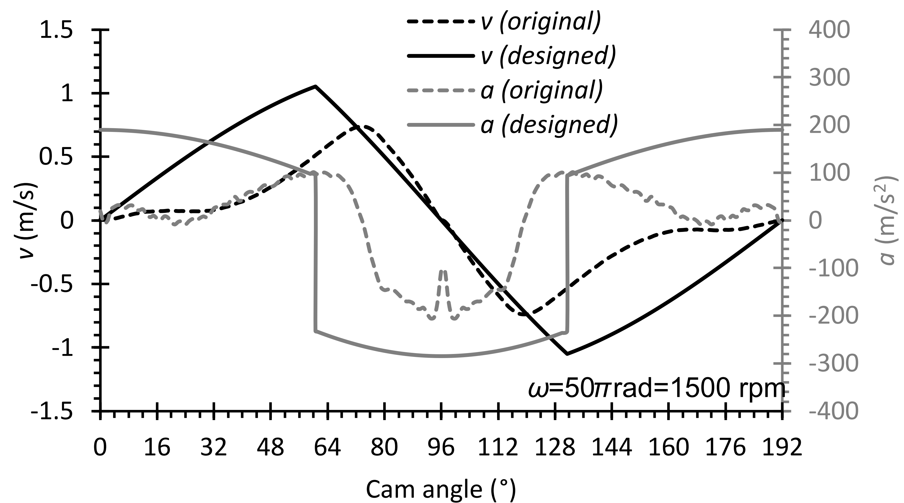
(b) Four stroke, exhaust follower
