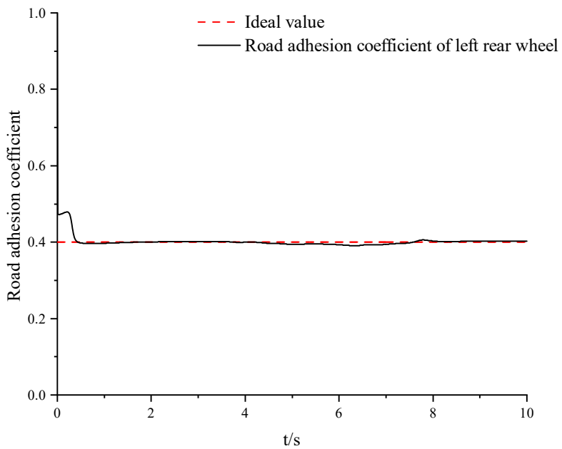
(c) Road adhesion coefficient of left rear wheel
