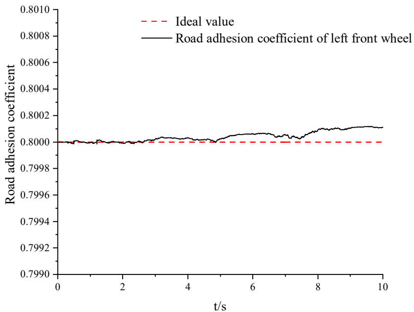
(a) Road adhesion coefficient of left front wheel
