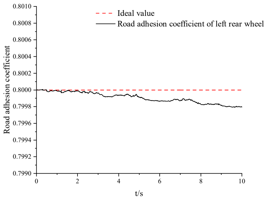
(c) Road adhesion coefficient of left rear wheel
