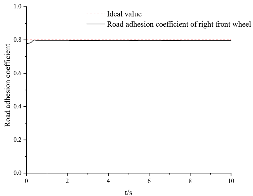
(b) Road adhesion coefficient of right front wheel
