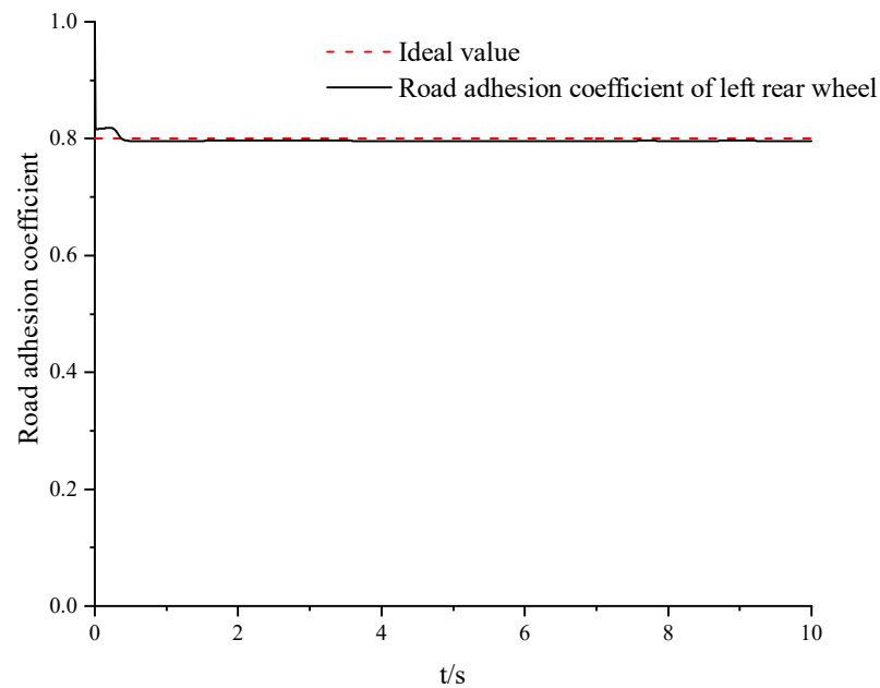
(c) Road adhesion coefficient of left rear wheel
