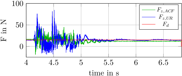
(a) v_d = 0.90 \text{ m s}^{-1} , F_d = 15 \text{ N}
