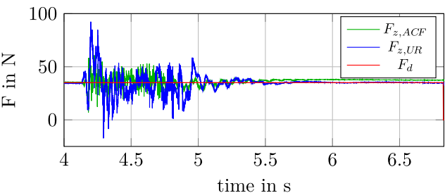
(b) v_d = 0.90 \text{ m s}^{-1} , F_d = 35 \text{ N}
