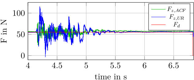
(c) v_d = 0.90 \text{ m s}^{-1} , F_d = 55 \text{ N}
