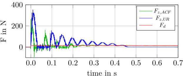
(b) Transient oscillation - Detailed View
