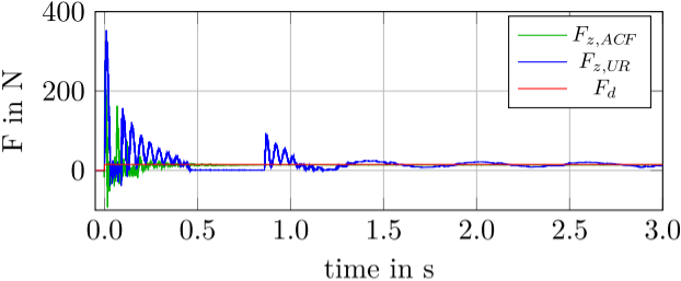
(a) Transient oscillation
