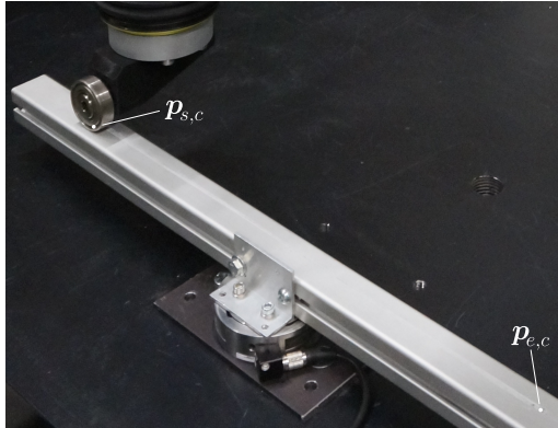
(a) Reel on straight profile
