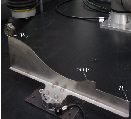
(a) Reel on ramp profile
