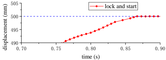
(a) displacement
