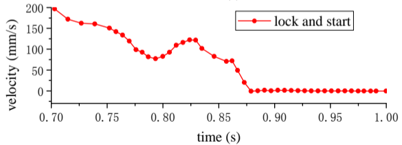
(b) velocity
