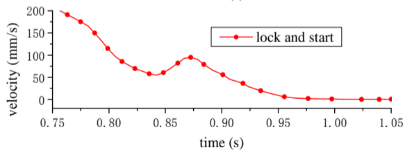
(b) velocity
