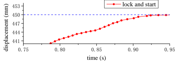
(a) displacement
