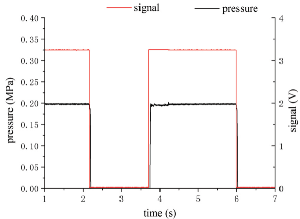
(b) pressure curve
