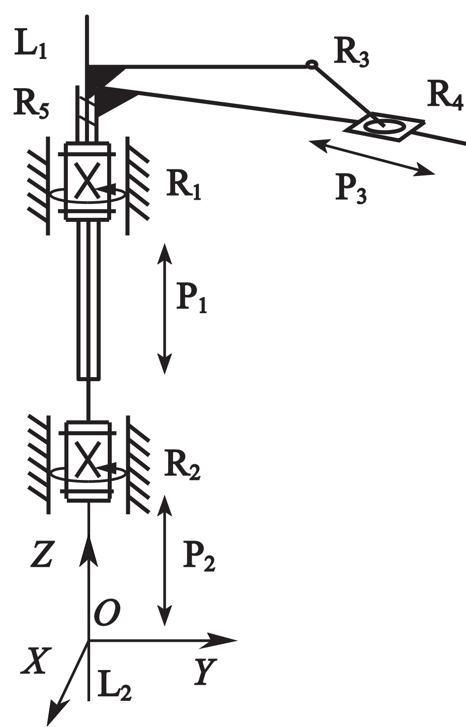
(b) The sketch of limbs and coordinate frame of equivalent architecture
