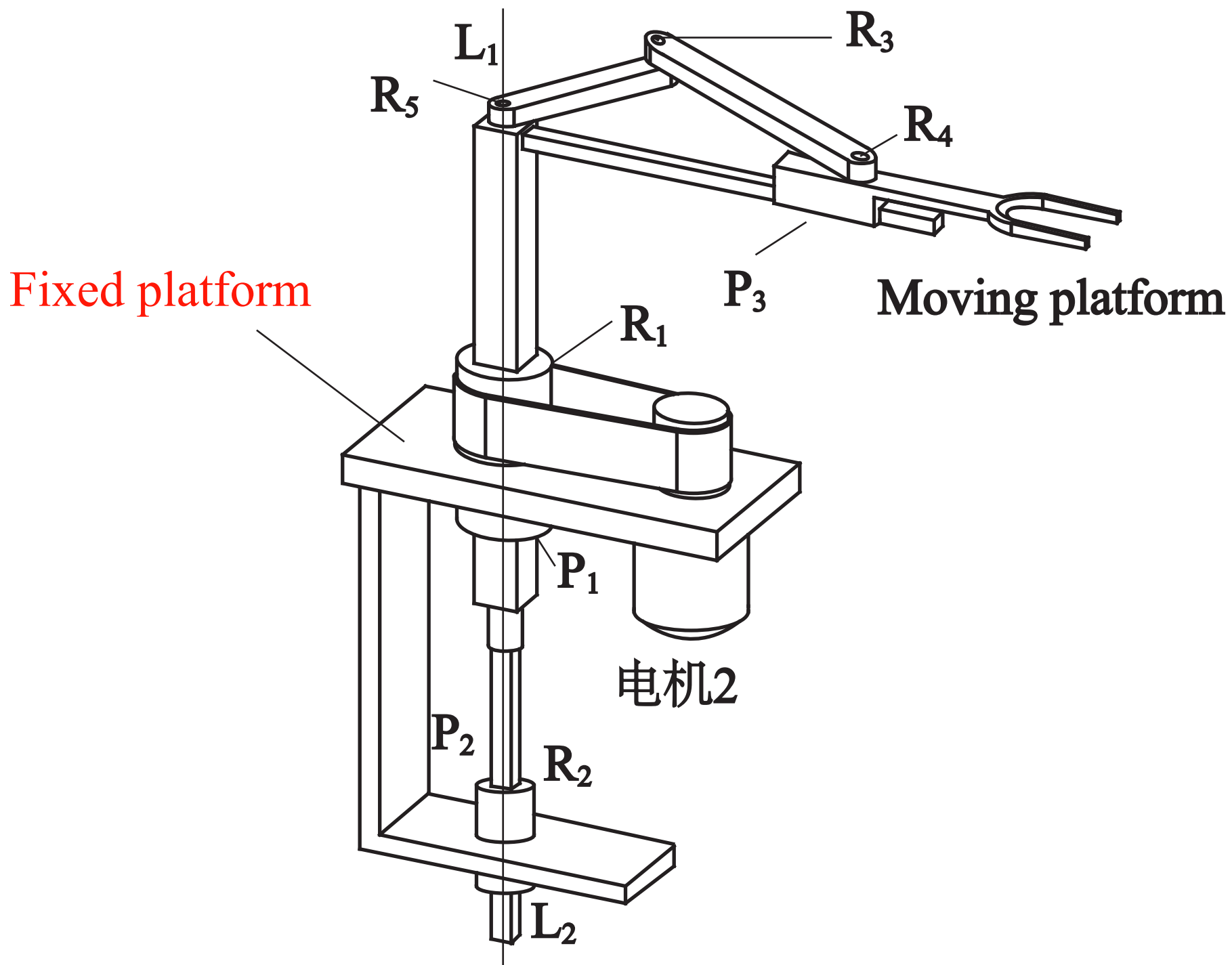
(a) Equivalent architecture
