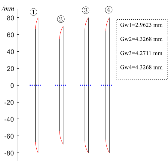
(a) Grinding wheel for generating i flank
